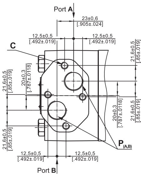
Side Ports
